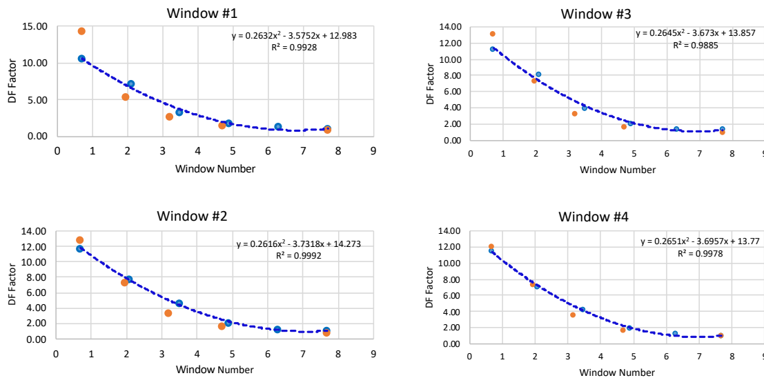
Figure 4: Evaluation of daylight factor at each window in both simulation by ALFA and physical model. The calibration also exhibits in (Figure 5) with 0.988963 correlation and 1.0536 calibration factor.
