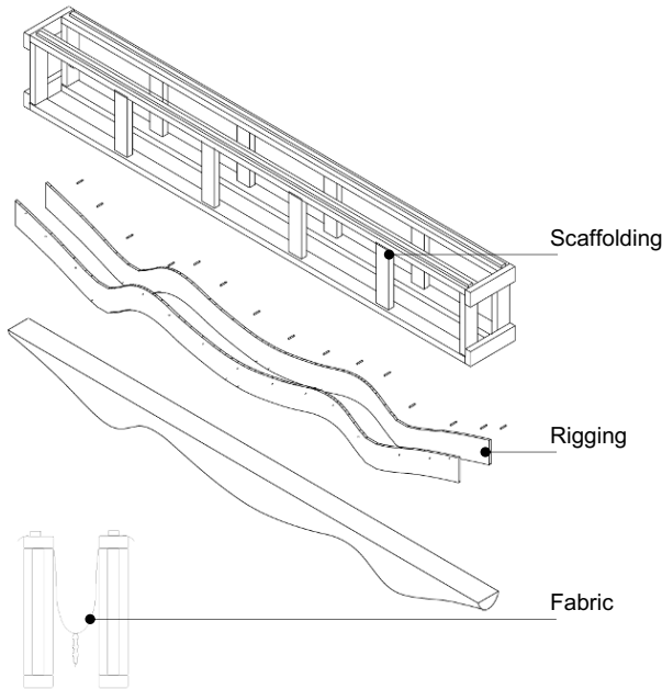
Figure 3: Formwork components.
