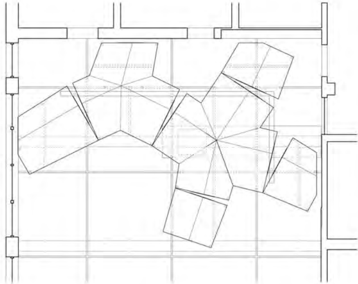
Figure 7: Reflected ceiling plan. Source: (Author 2019)
