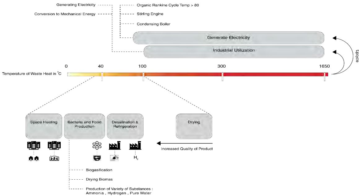
Figure 4: Common waste heat utilization processing based on temperature range (drawn by Sara Ghaemi based on Parker & Kiessling 2016; Juhara et al. 2018; Kocer 2004)
