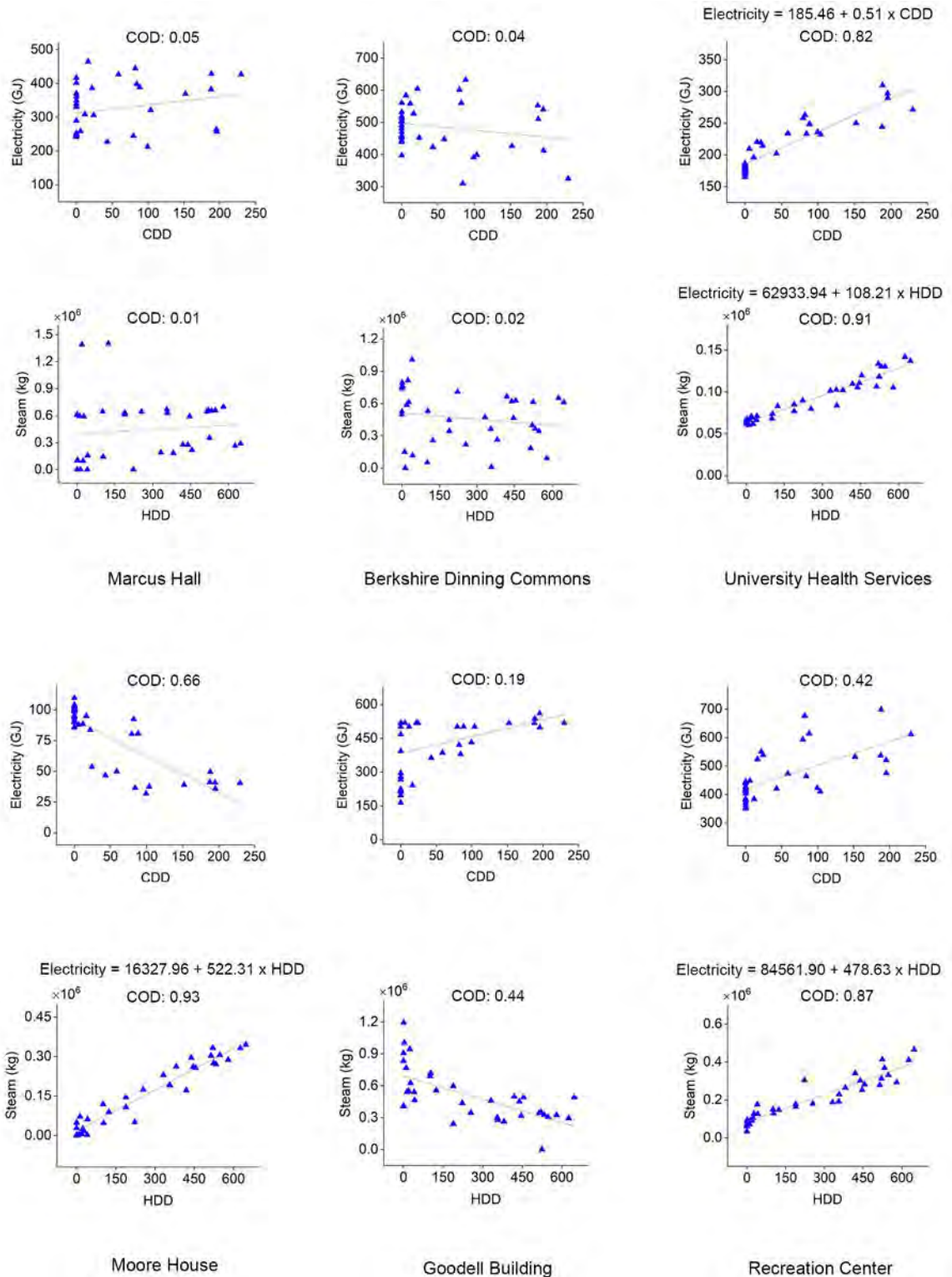
Figure 2: Case study buildings' energy vs. degree-days regressions.
