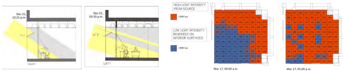
Figure 8: Challenges of the daylighting situation in the space, daylight glare presence due to the variations in windows' luminance values at sunny portions versus shaded portions (first and second images from left), under-illuminated areas <300 lux (third image from left), and over-illuminated areas >500 lux (last image on the right). Source: authors.
