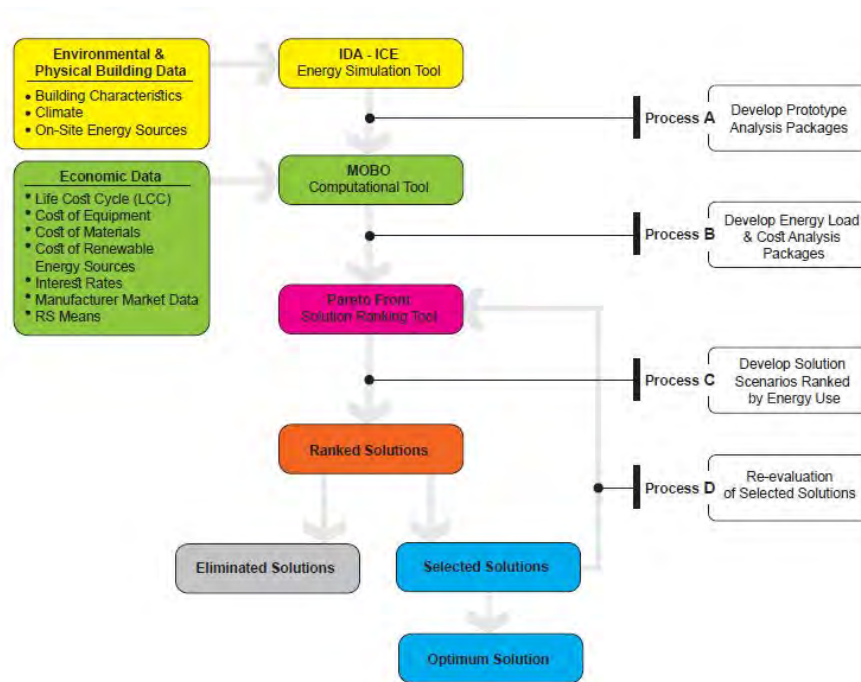
Figure 1: Methodology to optimize NZEB.
