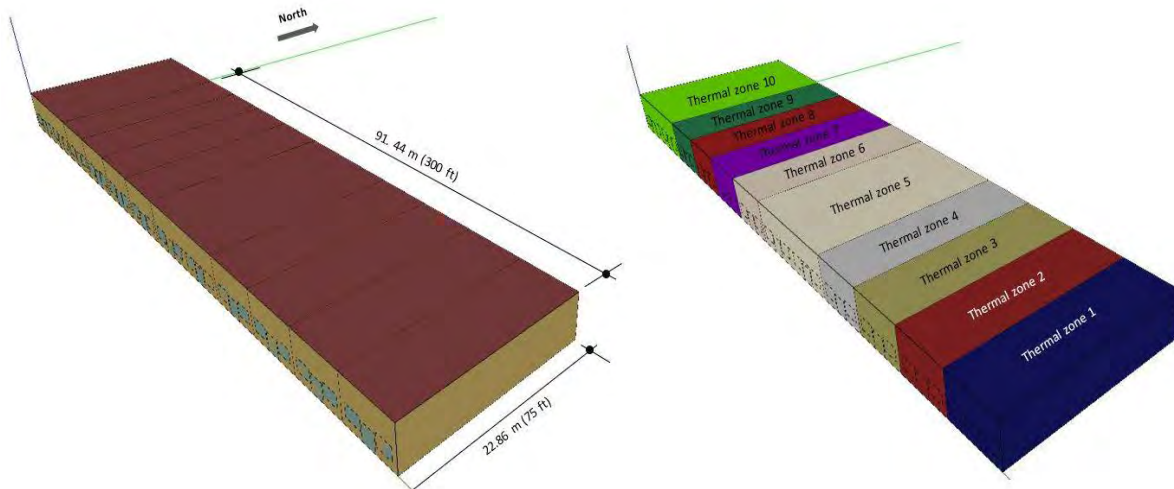
Figure 2: Simulation model of strip mall. (a) Building dimensions. (b) Thermal zones (Each store is considered as one thermal zone)
