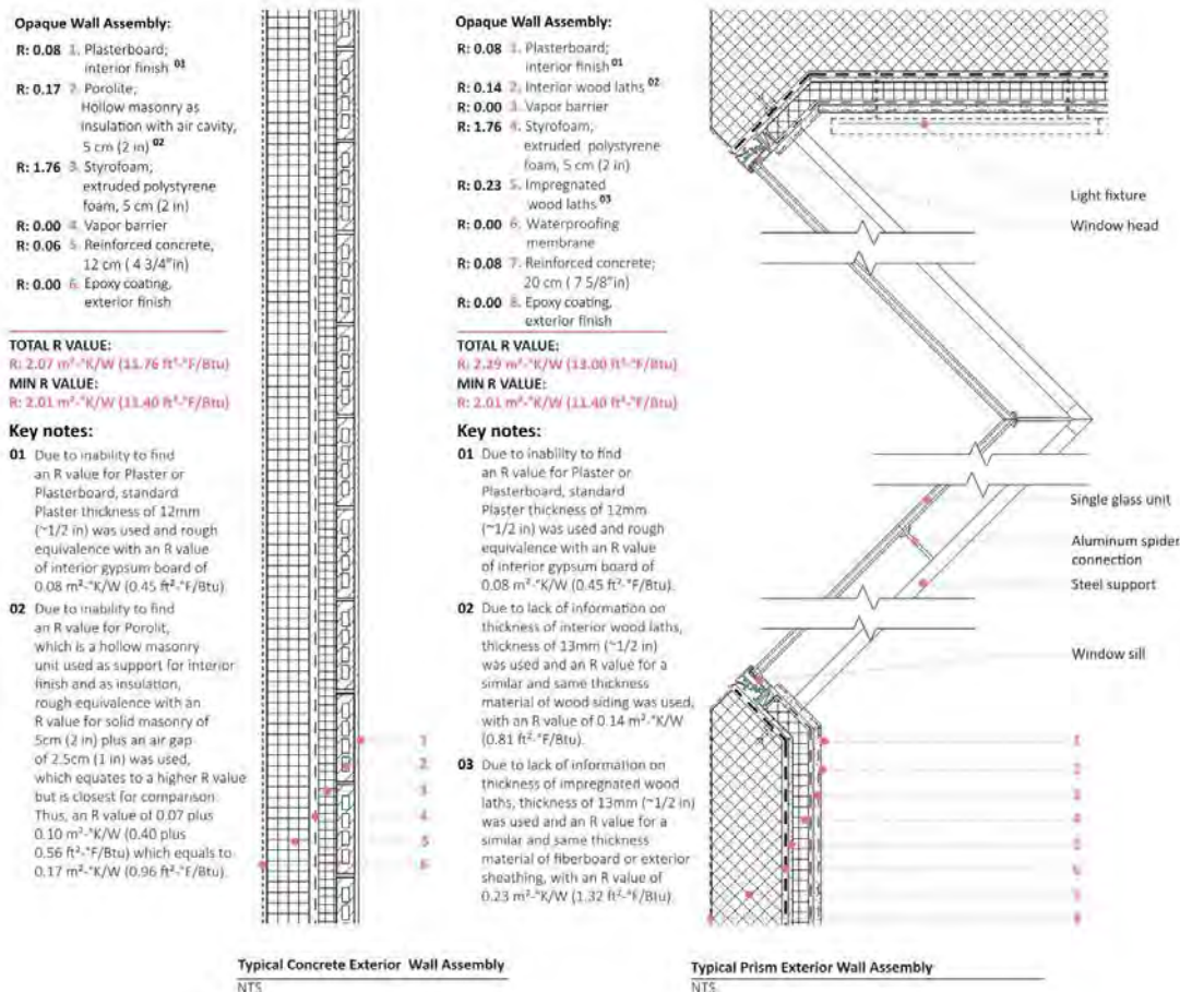
Figure 8: Thermal performance analysis of two selected exterior wall assemblies at Spomen Dom.
