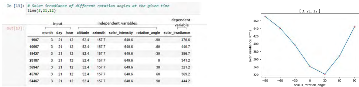
Figure 4: Data table containing information on independent and dependent variables (left) and visualized results of solar irradiance values of varying rotational angles at 12 PM on March 21st (right) (Author, 2021)
